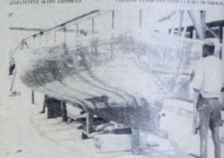
TOP: A ferro-cement boat rigged out as a simple yacht, and BELOW: A ferro-cement boat in formation, with the steel frame being carefully covered with layers of wire mesh, prior to being plastered with cement.
