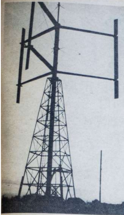
SPACE-AGE WINDMILL. A new generation of windmills has been born. The unit, designed by the U.S. McDonnell Douglas company is different to former windmills because its vertical blades rotate horizontally. Due to extensive testing at Rocky Flats, Colorado, the invention, called Giromill, will produce enough power for 15 homes. PHOTO: KEYSTONE
