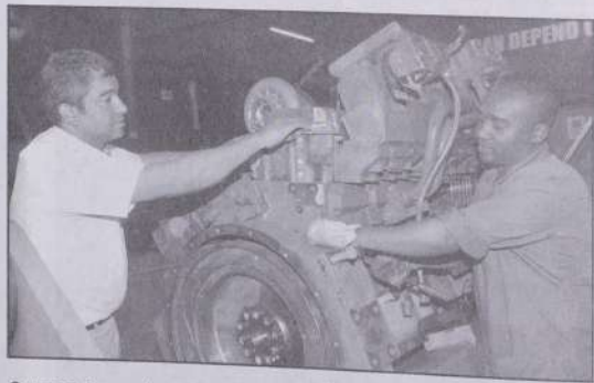
Car and General engineers have the major task of rebuilding a giant Cummins 30,000cc engine at the Company's High Horsepower Engine Rebuild Centre in Lusaka Road. Randall Truter (left), the Cummins High Horsepower Workshop Manager and Joseph Kibunja (right), the Assistant Divisional Field Service Engineer, repair the engine belonging to a power generation company in Tanzania.
