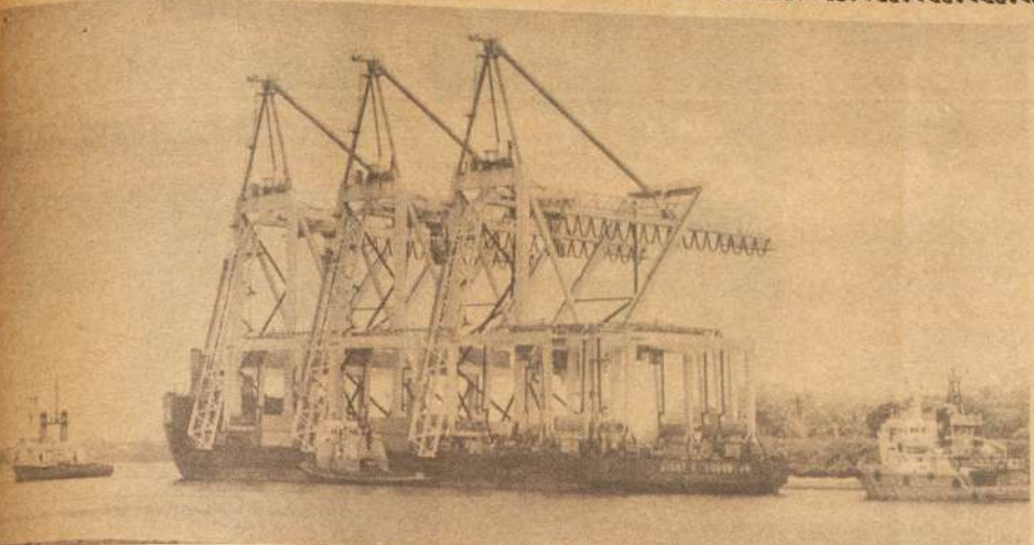
TUGS surround the 'Giant Four' as she enters Kilindini with her cargo of huge gantry cranes. PHOTO: NATIONAL STUDIO
